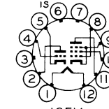
12FM 6T9
